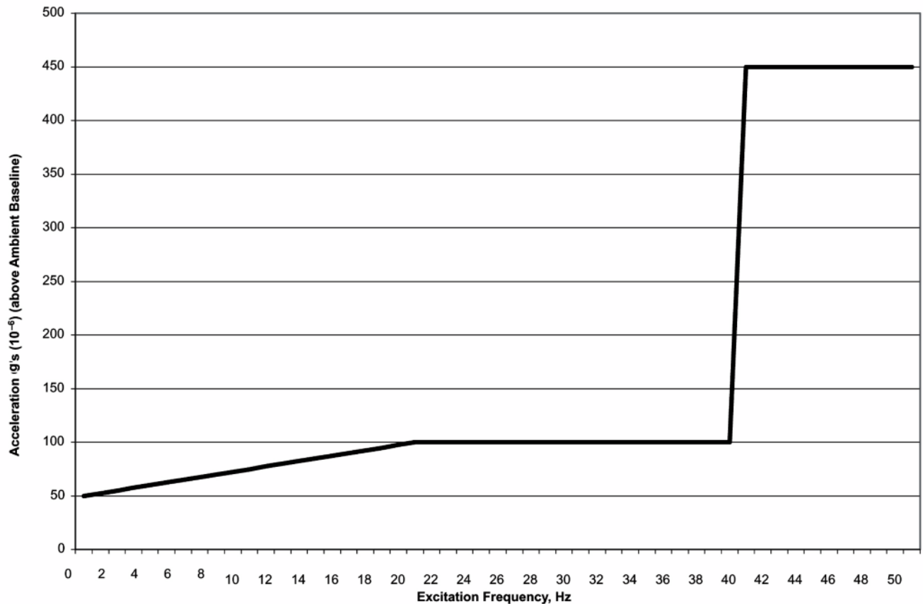
Illustration 5-10: 1.5T LCC Magnet Steady State Vibration Specifications
