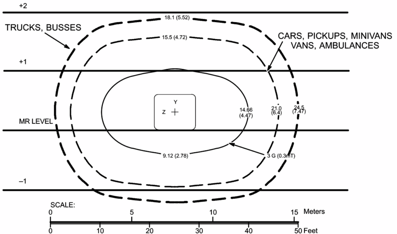
Illustration 5-8: Magnet Moving Metal Sensitivity Line Plot (Vertical View)
