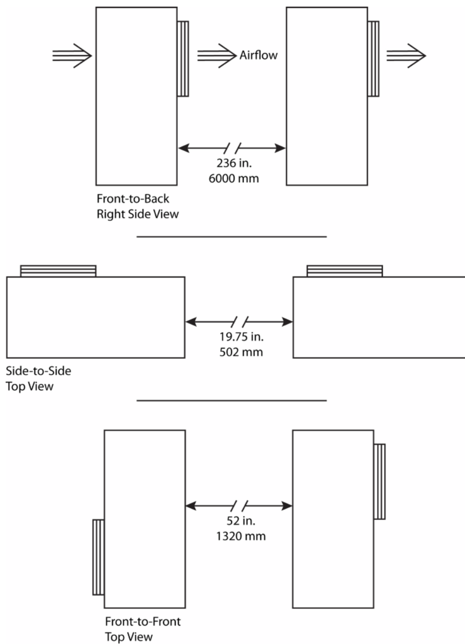
Illustration 8-10: Required Configurations and Separation Distances for Multiple MRCCs
